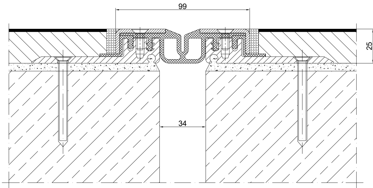
CONECTO GA 50.20.25 S SECTION
