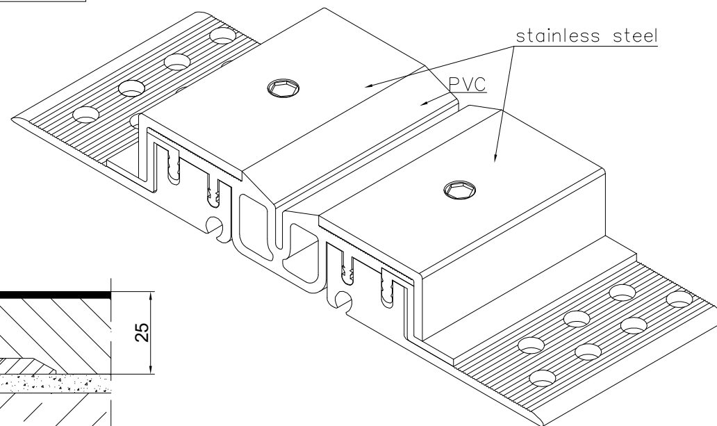
CONECTO GA 50.20.25 S VIEW
