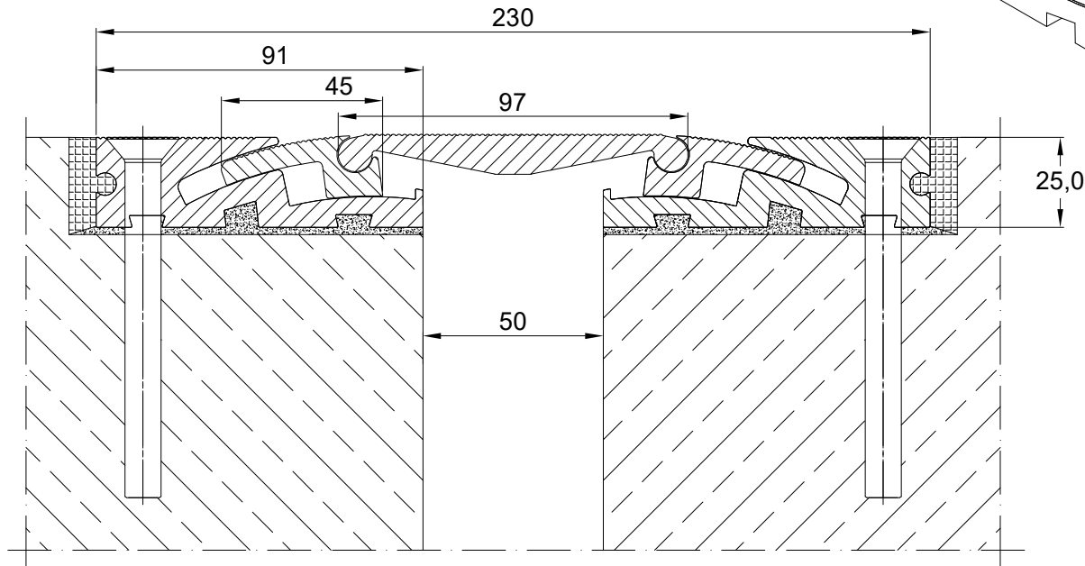
CONECTO HDS 230.20.25 SECTION
