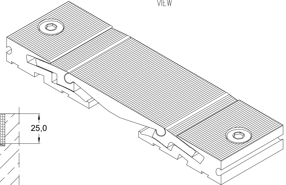
CONECTO HDS 230.20.25 VIEW
